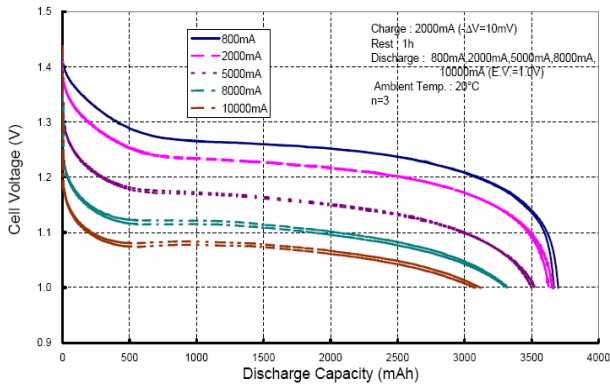
Fig. 1 Discharge Profile-Rate
