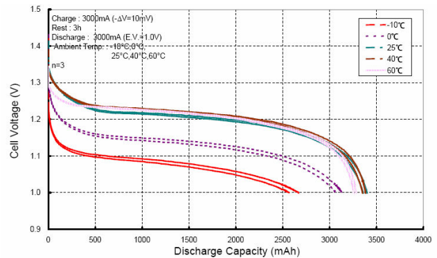
Fig. 2 Discharge Profile-Temperature
