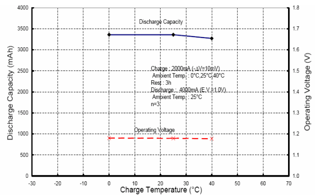
Fig. 4 Charge Temperature Characteristic
